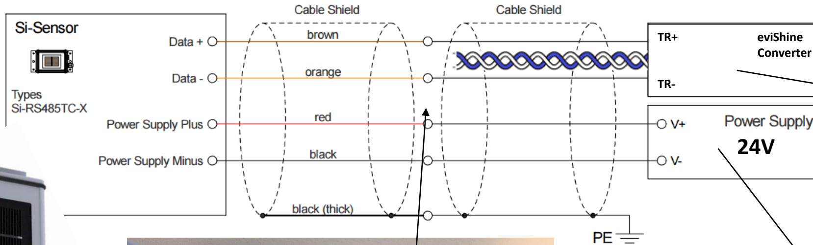
Wiring diagram of digital Si sensors
